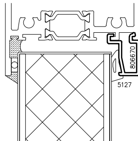
2" Panel Inside Glazed
