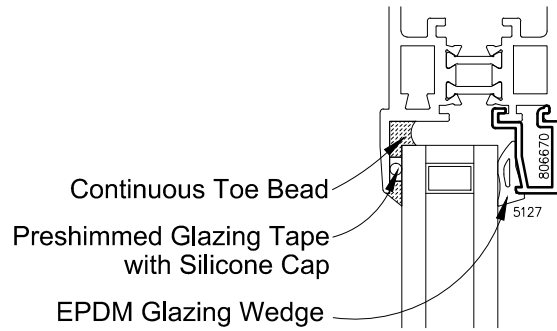
1" Insulating Glass Operable Inside Glazed
