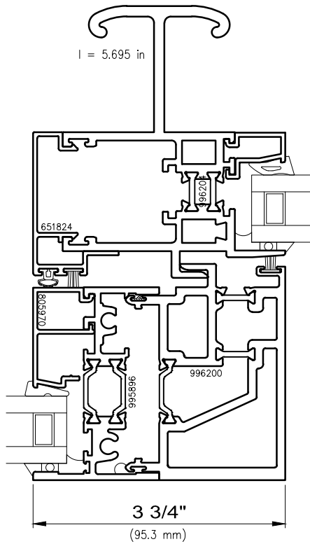
6 Meeting Rail Inside Slide
