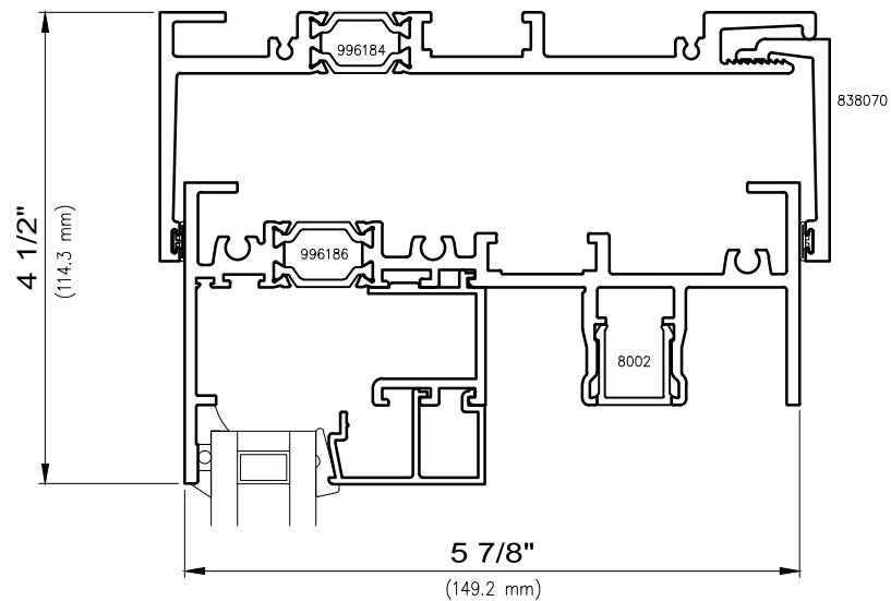
① Fixed Head Inside Slide
