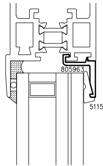
1-3/8" Insulating Glass Operable Inside Glazed
