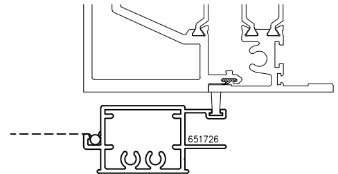
Meeting Rail
