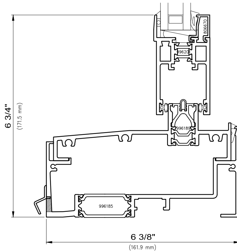
4 Operable Sill Inside Slide
