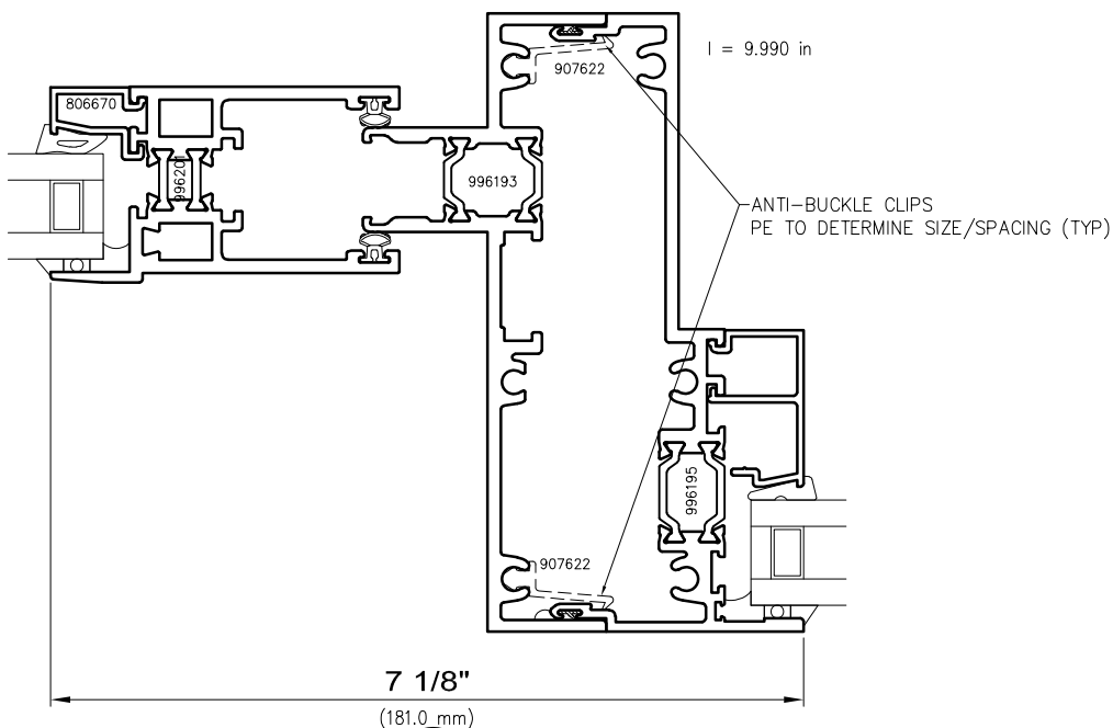
10 Operable/Fixed Stack Inside Slide
