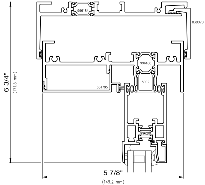
3 Operable Head Inside Slide
