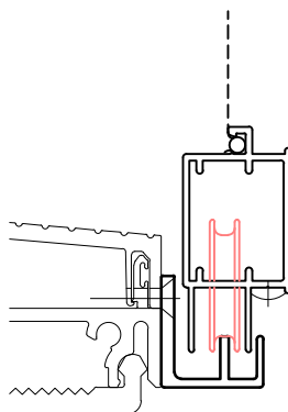
Sill
