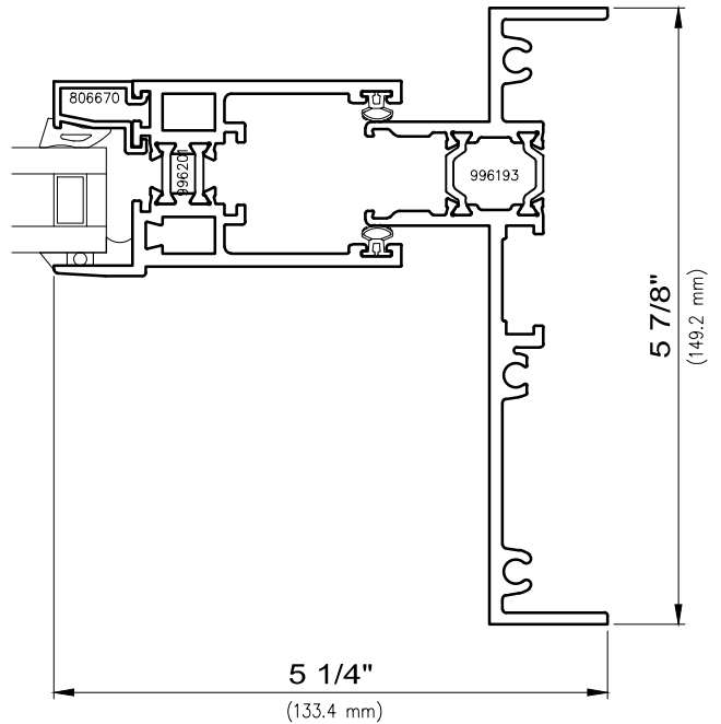
5 Operable Jamb Inside Slide
