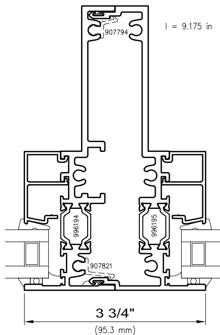
9 Fixed/Fixed Stack Inside Slide
