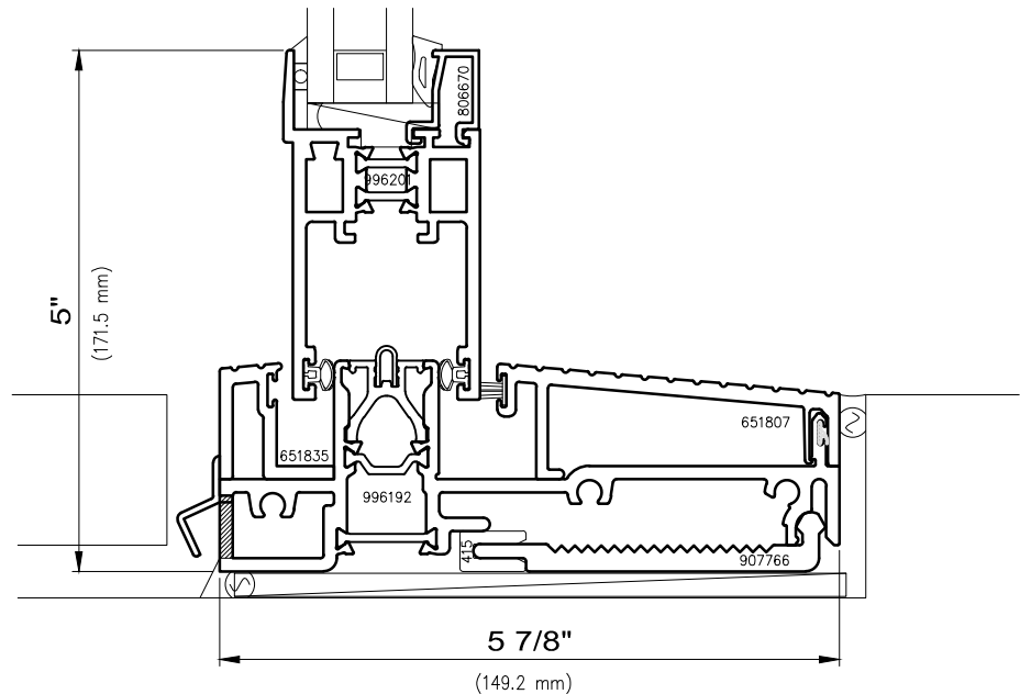
16 Operable Sill Outside Slide
